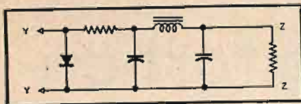
Fig. 4. Rectifier and low-pass filter circuit.
