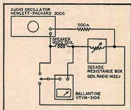
Fig. 7. Circuit used to make impedance measurements.
