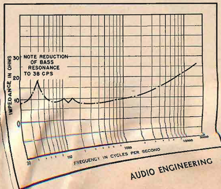
Fig. 6. Impedance curve of GE S-1201 D speaker mechanism in Super Horn.
