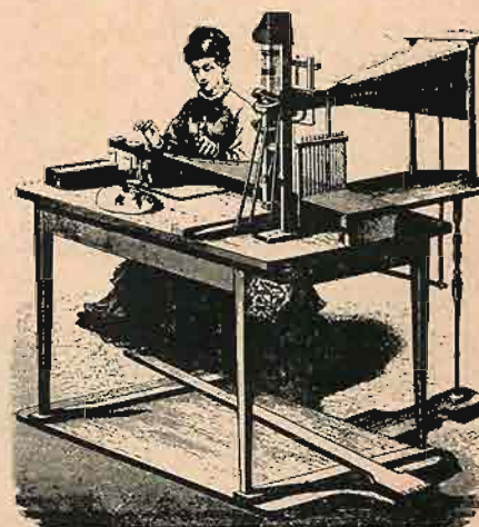
Fig. 7-4. The Faber speech organ. Intelligible speech could be "played" from the rubber lips in front of the bellows. From: Internationale Zeitschrift für Allgemeine Sprachwissenschaft , 1884.
