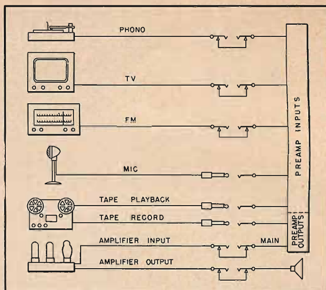
Fig. 4. Patch system functions as distributor-head for entire system, giving it complete flexibility and permits semi-automatic operation from owner's couch.
