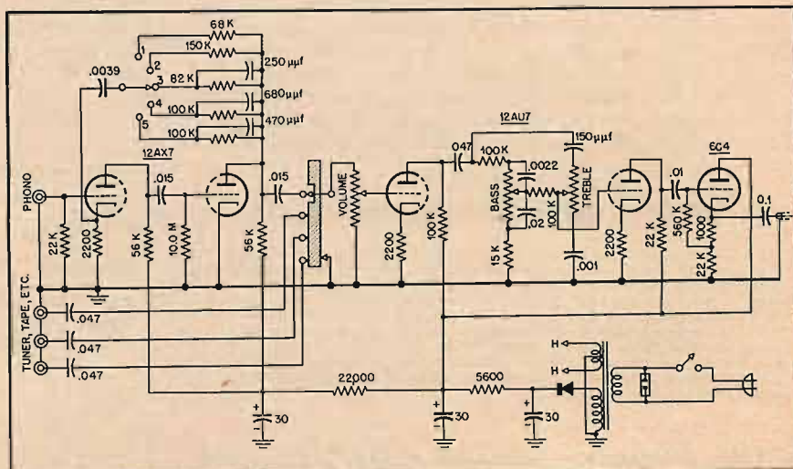
Fig. 2. Schematic of the new Tech-Master kit as observed from a pre-production model.
